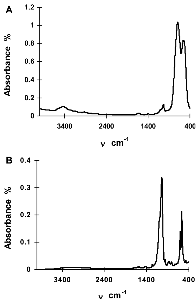
Fig. 3 Fourier transform (FT) IR absorption spectra of a OCP crystals nucleated on \text{TiO}_2 anatase particles and of b reference hydroxyapatite (HAP, Merck)
