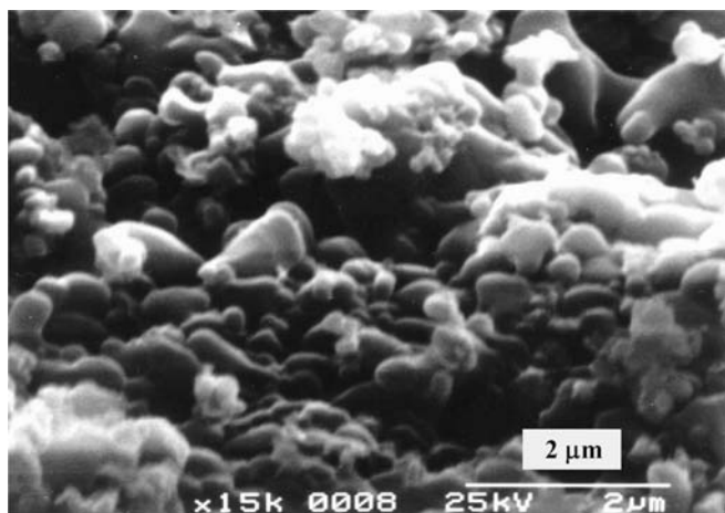
Fig. 5 Scanning electron microscope image of HAP on TiO 2 anatase particles at \times 15,000 magnification
