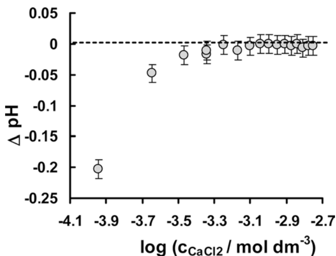
Fig. 1 pH change in titania suspension ( 0.5 \text{ g } 200 \text{ cm}^{-3} , pH 6.8) in 0.05 \text{ M NaCl} due to addition of \text{CaCl}_2 solution. The dotted line designates the pH value of 6.8, to which the pH was reset after each \text{CaCl}_2 portion
