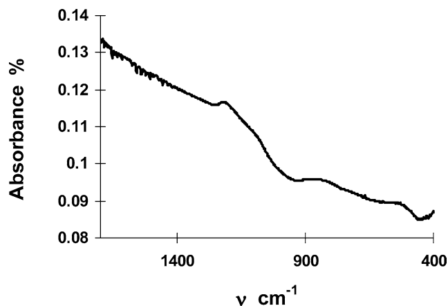
Fig. 7 FT-IR spectrum of calcium phosphate deposited onto an evaporated titanium layer
