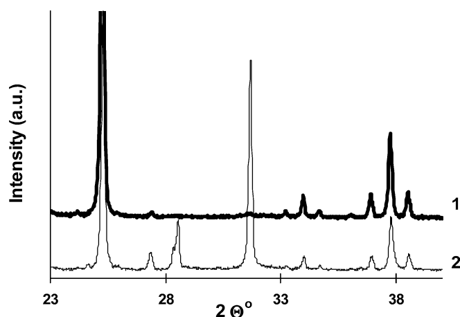
Fig. 4 X-ray diffraction pattern of OCP crystals (1) and HAP crystals (2) nucleated on \text{TiO}_2 anatase particles
