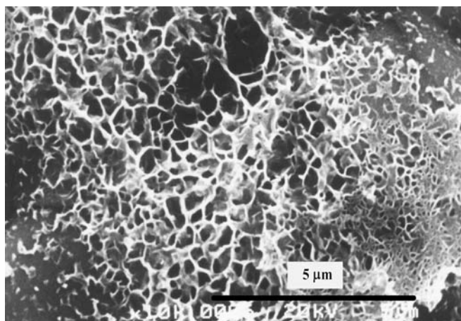
Fig. 9 Scanning electron microscope image of calcium phosphate nucleated on the surface of a titanium plate pretreated by laser ablation and heating at 450 °C for 3 days
