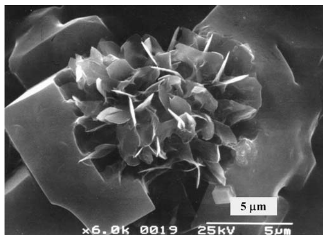
Fig. 2 Scanning electron microscope image of octacalcium phosphate (OCP) crystals on \text{TiO}_2 anatase particles at \times 6,000 magnification
