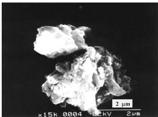
Fig. 6 Scanning electron microscope image of a calcium phosphate deposit on an evaporated titanium layer at \times 15,000
